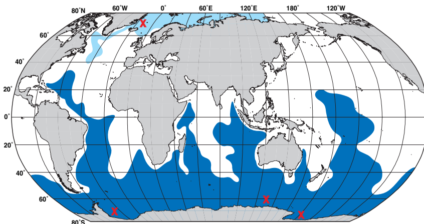
Fig. 7 A representation of the spread of Antarctic Bottom Water (AABW, dark blue, based on the \sigma_4=45.92 kg/m 3 density surface). From [Talley, 1999]
