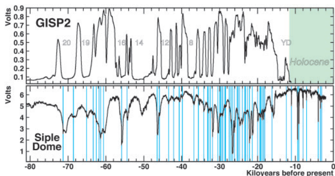
Fig. 1. Scattering on the higher dust concentrations that accompany cold periods increases the dust-logger signal in a profile of the clear ice at GISP2 ( Upper ), whereas absorption on dust decreases signal in the bubbly ice at Siple Dome ( Lower ). The GISP2 data have been smoothed for clarity; a few interstadials and the Younger Dryas (YD) are labeled. Volcanic signatures at Siple Dome are indicated with hashing; when magnified, each signal (here distorted in age space) is a distinctive asymmetric double spike (see, for example, the cusp near 71 ka).
