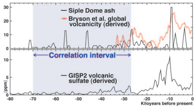
Fig. 4. Comparison of our Siple Dome ash record with the global volcanicity index of Bryson and Bryson (13) ( Upper ) and the GISP2 volcanic sulfate of Zielinski et al. (15) ( Lower ), each averaged over 1 kyr. The Siple Dome ash magnitude ranking is from ref. 6; the Bryson volcanicity index has been renormalized. The Bryson curve does not extend back beyond 35 ka because of the limitation of radiocarbon dating. All three curves indicate that the greatest activity was \approx 10 ka during the main deglaciation of the early Holocene.
