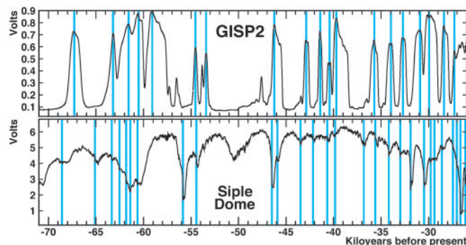
Fig. 2. Interval over which the correlation was calculated, with hashing to indicate Siple Dome volcanic events ( Lower ) and GISP2 DO cold events ( Upper ). For clarity, a few of the weakest volcanic events are not indicated. The stadial near 67 ka has been associated with the Toba supereruption (28).
